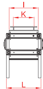
TAIL SECTION
