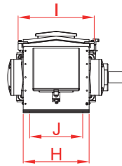
HEAD SECTION
